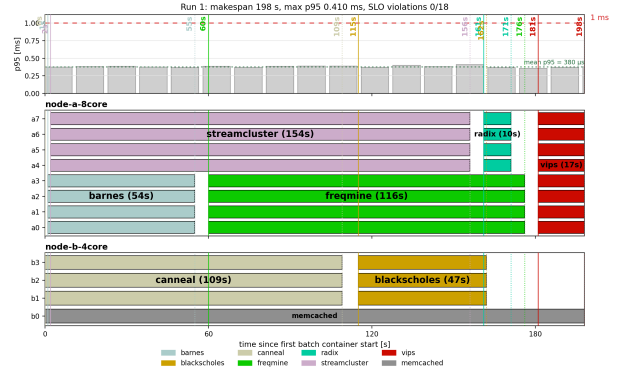
AI-generated policy run: makespan 198s, max p95 409.9 \mu s, SLO violations 0.
