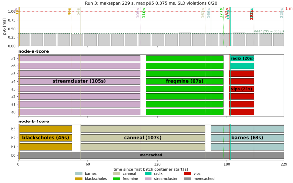
Handcrafted comparison run: makespan 229s, max p95 375.2 \mu s, SLO violations 0.
